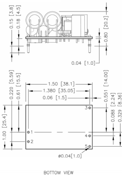
43MAC-D Pin Type
