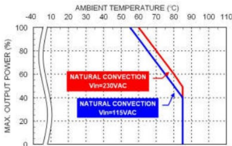
Derating Curve vs. Ambient Temperature MAC15USxxB xx=3P3/05/7P5/09/12/15/18 Connector Option : (Blank: JST)
