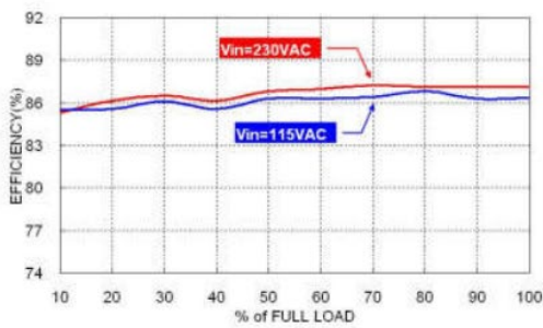
MAC15US12B Efficiency vs. Output Load
