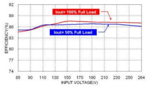
MAC15US12B Efficiency vs. Input Voltage
